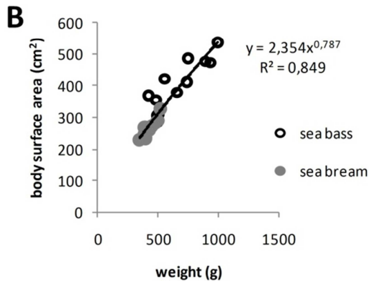
Figure 4. Body surface area. A: Mosteller's formula against actual body surface area. The plot shows a good agreement between the Mosteller's formula and the body surface area, but the best fit power-model ( y ) was not right linear. Mosteller's formula = M^{1/2} \cdot h^{1/2} , M = body mass, h = body length. B: body surface area against body weight. The best fit power-model ( y ) showed a power of 0.79, close to relation (6) and to that proposed by Kleiber (1932).
